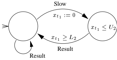
Figure 6: Hybrid Automaton from Formula S_{\text{Mode}} in Figure 3
