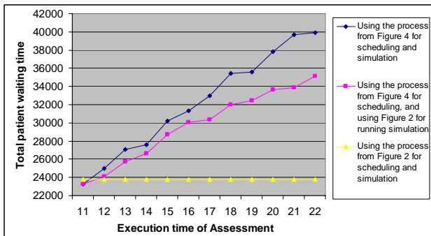
Figure 5. Total waiting time of less precise process under different execution time of assessment
