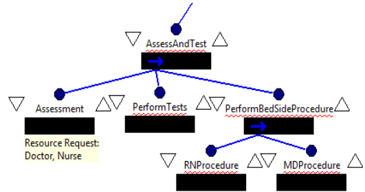
Figure 4. ED process with less precise details
