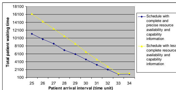
Figure 6. Total waiting time using precise and less precise resource descriptions
