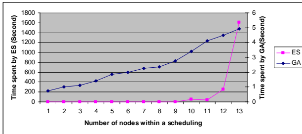
Figure 8. Scheduling time comparison of GA and ES
